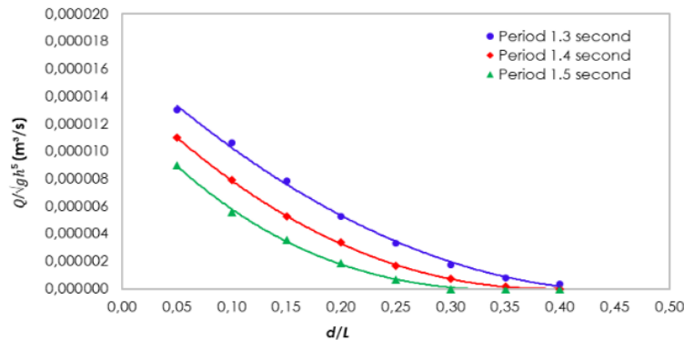
Fig 10: Relationship of d/L with Q/\sqrt{gh^5}
