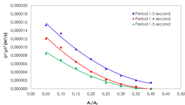
Fig 7: Relationship of A_1/A_2 with Q/\sqrt{gh^5}
