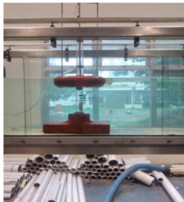
Fig 4: In-channel wave pump model
