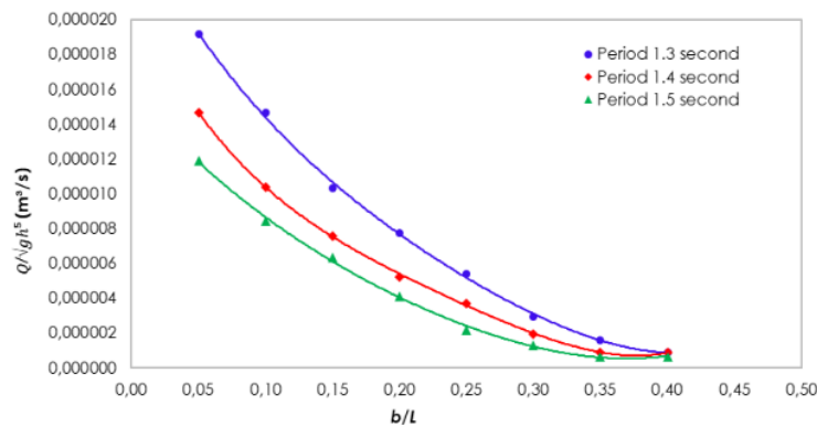
Fig 9: Relationship of b/L with Q/\sqrt{gh^5}
