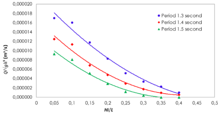
Fig 8: Relationship of H_i/L with Q/\sqrt{gh^5}
