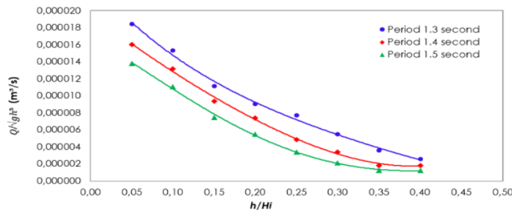
Fig 11: Relationship of h/H_i with Q/\sqrt{gh^5}
