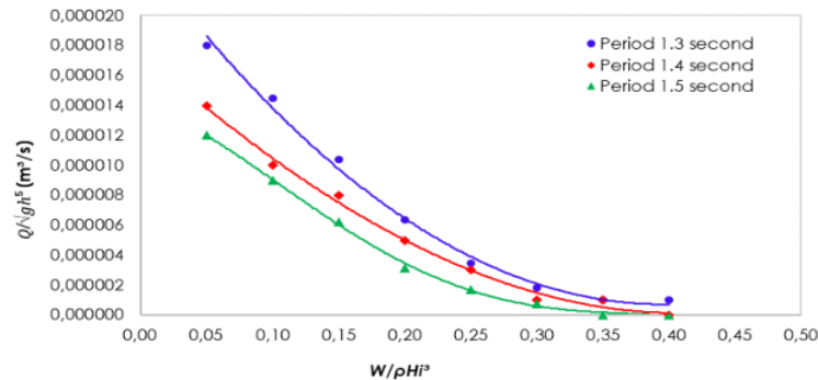
Fig12: Relationship of W/\rho H_i^3 with Q/\sqrt{gh^5}
